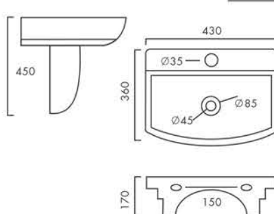
TERUS Design No.: 6003
