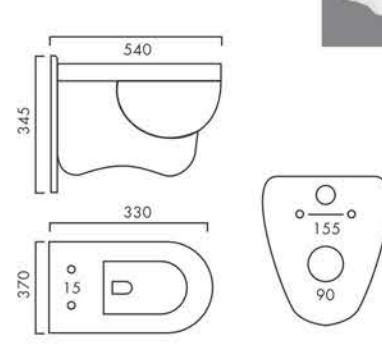
SPARKLE Design No.: 2004
