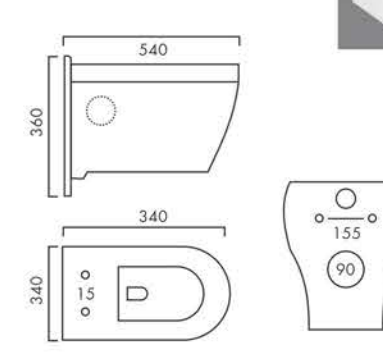
ASTA Design No.: 2008
