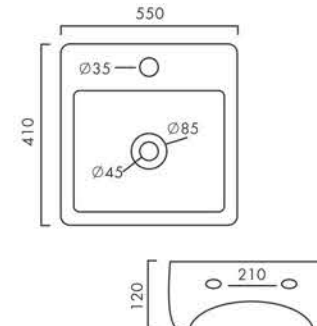
DELUXE CORNER Design No.: 3058
