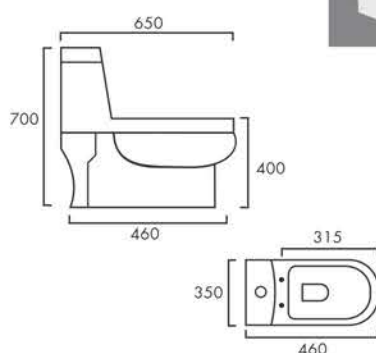
BREZZA Design No.: 1006
