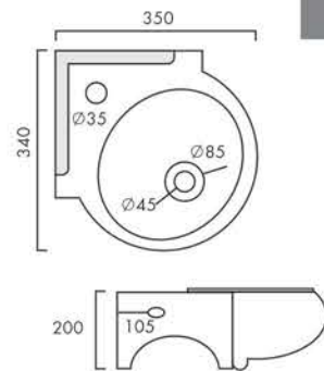
GRESS Design No.: 3005
