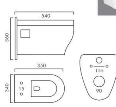
ARCTIC Design No.: 2010
