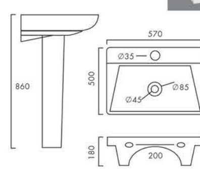
SERENA Design No.: 6007
