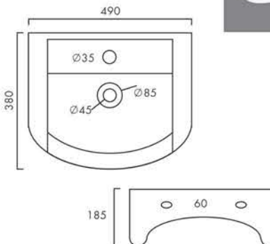
VIPRO Design No.: 3007
