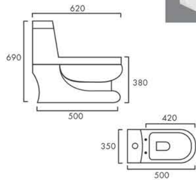
TERENO Design No.: 1001
