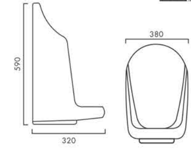
LEDI URINAL Design No.: 7055
