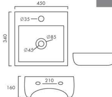
CORUS Design No.: 3057
