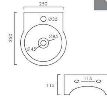
POLOK Design No.: 3055
