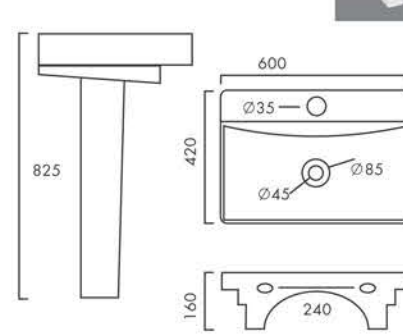
SOFTYA Design No.: 6009
