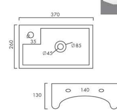
CORUS Design No.: 3057
