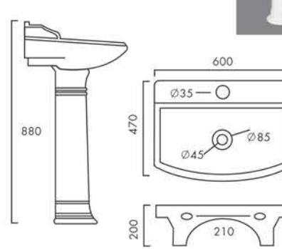
SERENA Design No.: 6007
