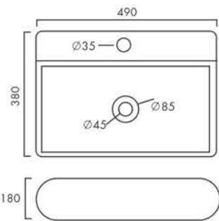
ASTAR Design No.: 5051
