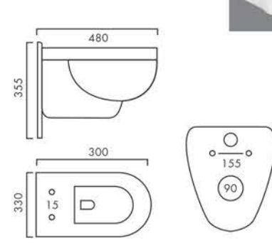
GLORY Design No.: 2001
