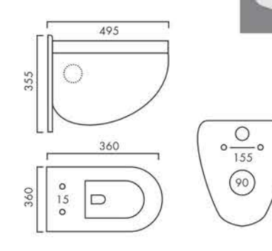
SARA Design No.: 2005
