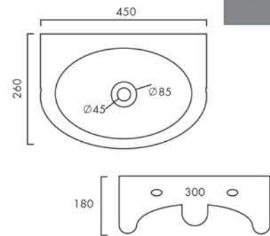
SMART Design No.: 3004
