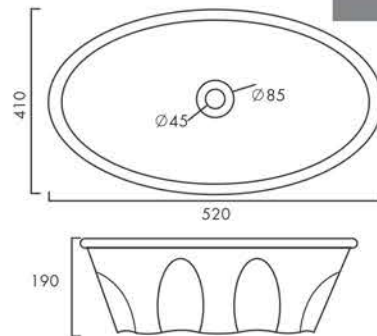
LYRA HALFSET Design No.: 5053
