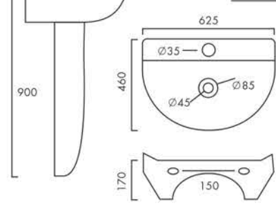
LEO Design No.: 6014
