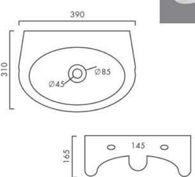
BRITANIC Design No.: 3009
