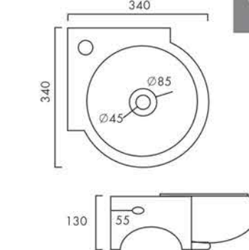
DELUXE CORNER Design No.: 3058
