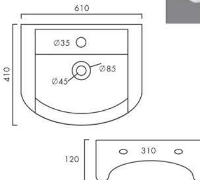
ATLANTA Design No.: 3010
