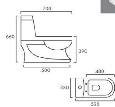
CROMA Design No.: 1003
