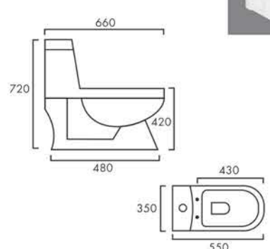
VENUS Design No.: 1007
