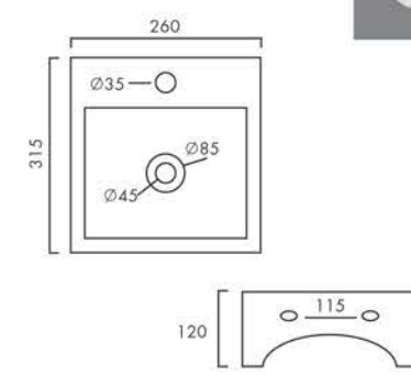
SPARK Design No.: 3054
