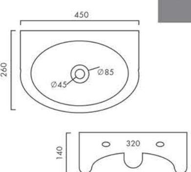
ALVIN Design No.: 3008
