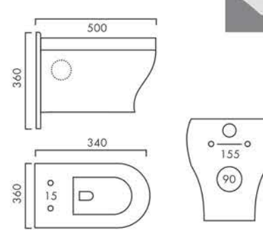
ARCELLA Design No.: 2006
