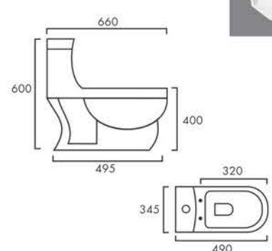
SYPHONIK Design No.: 1010
