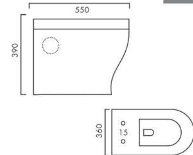
ANGLO Design No.: 7004
