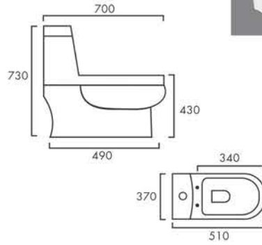
BLACK PEARL Design No.: 1011
