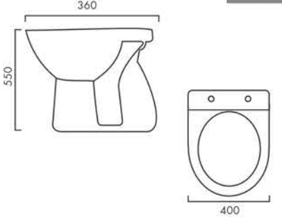
MINTO Design No.: 7051
