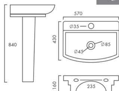
SWISS Design No.: 6002
