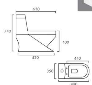
ROMANO Design No.: 1004
