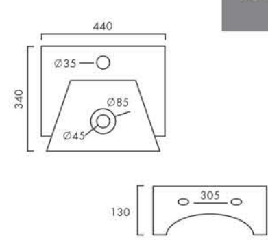
MATIZ Design No.: 3011
