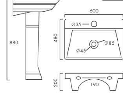
CIPLA Design No.: 6015
