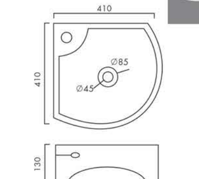
SCORE CORNER Design No.: 3056
