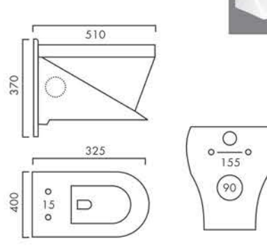
ZEST Design No.: 2009
