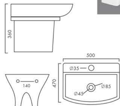
SWISS HALF SET Design No.: 5055
