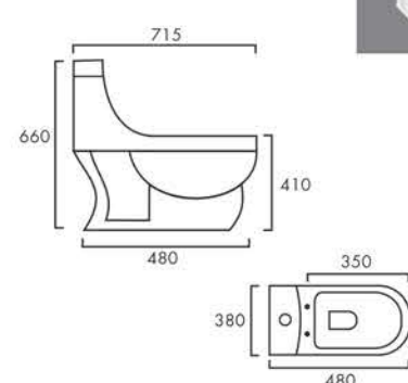
ATHENS Design No.: 1009
