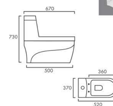
HAIRA Design No.: 1012
