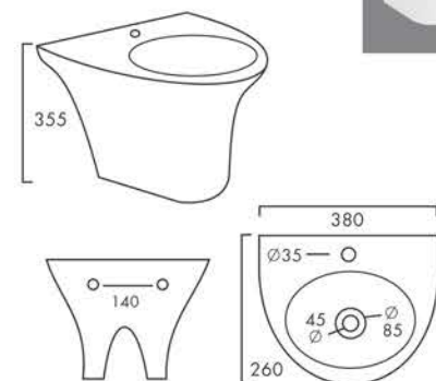
LYRA HALFSET Design No.: 5053
